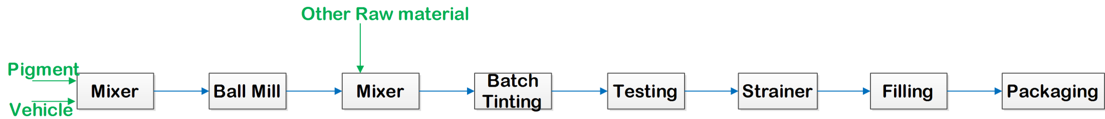
Figure: Manufacturing of Paint
